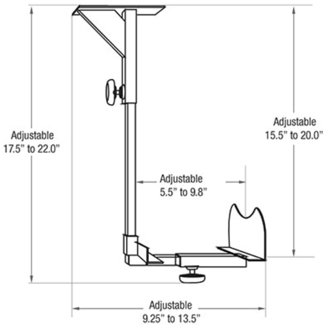
Vertical Configuration
