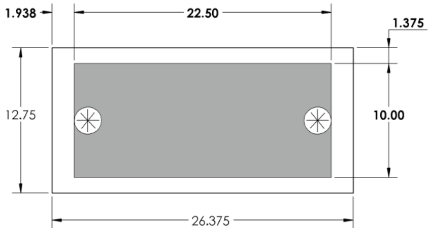
Console Top Removable Panel Cutout
