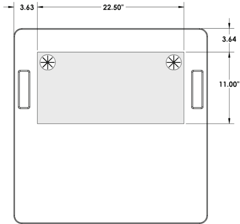
Work Surface Cutout
