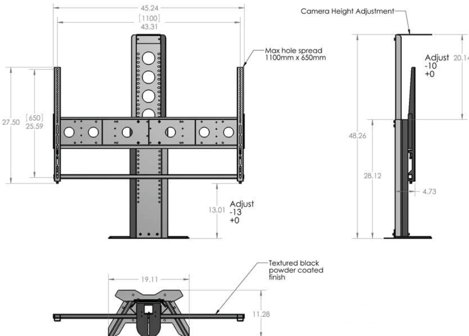
Shown installed on the PL3070 cart (sold separately)
